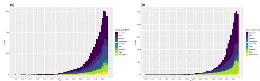
Figure 2: The trend of publications based on longitudinal omics studies within the last 8 decades in PubMed (panel a) and Scopus (panel b) databases.
